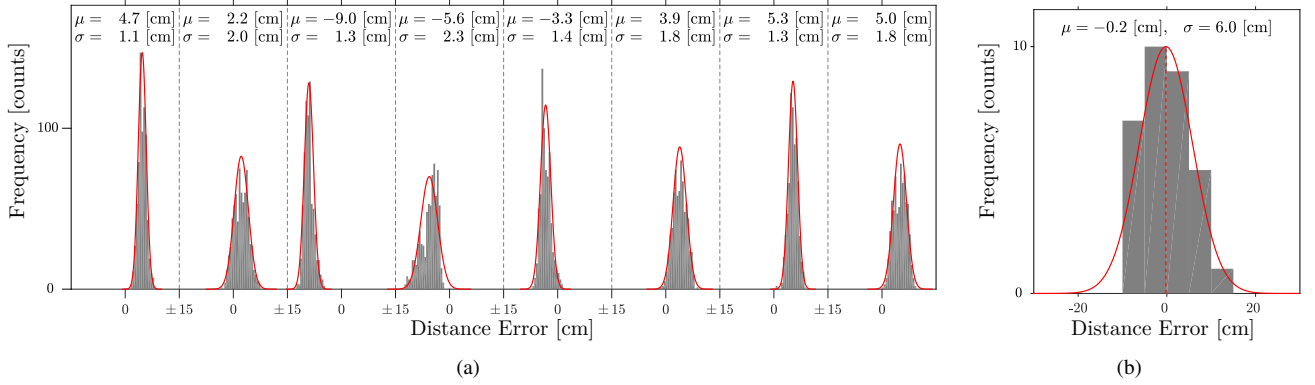
Fig. 3. (a) Experimental results showing the UWB distance errors measured between a tag and an anchor for eight different locations and orientations. Each histogram (gray) shows the error statistics of 800 two-way-ranging distance measurements for a particular distance between the devices, the red line shows the normal distribution with mean, \mu , and standard deviation, \sigma , of the data. (b) Error statistics of the mean-offset of 32 different distance and relative orientations of the same pair, i.e., the statistics of means from (a).
