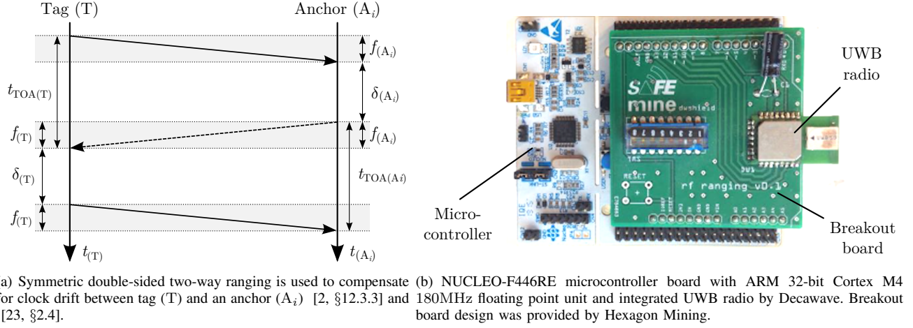
Fig. 2. Experimental implementation of an optimization-based localization system using off-the-shelf microcontrollers and UWB radios.
